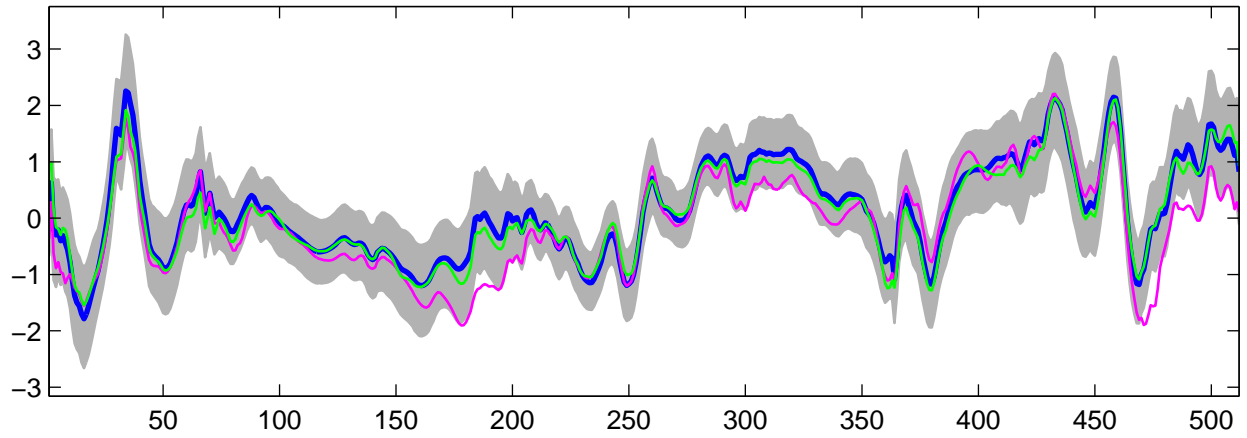
Estimated U_{28}(t) using G-WFMM: DE data, run 4
