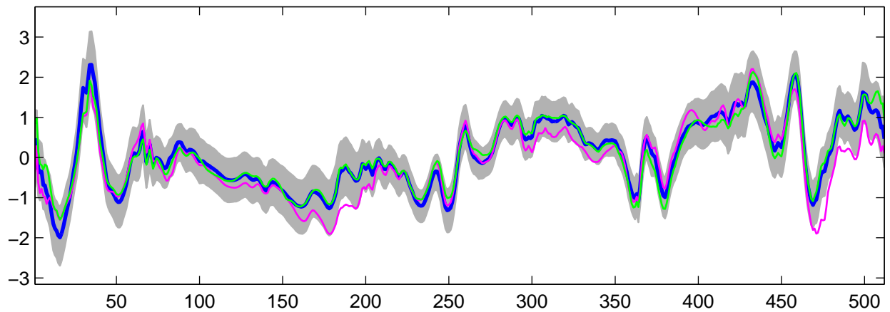
Estimated U_{28}(t) using R-WFMM: DE data, run 4
