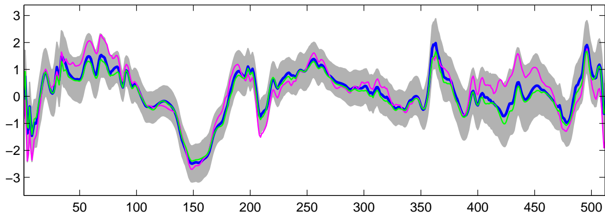
Estimated U_{28}(t) using G-WFMM: Normal data, run 4
