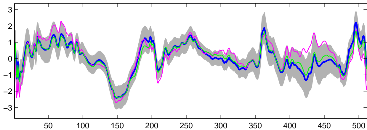
Estimated U_{28}(t) using R-WFMM: Normal data, run 4
