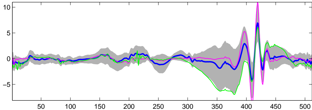
Estimated U_{28}(t) using G-WFMM: t_1 data, run 4
