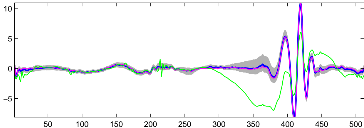
Estimated U_{28}(t) using R-WFMM: t_1 data, run 4
