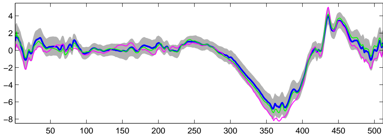
Estimated U_{28}(t) using G-WFMM: t_2 data, run 4
