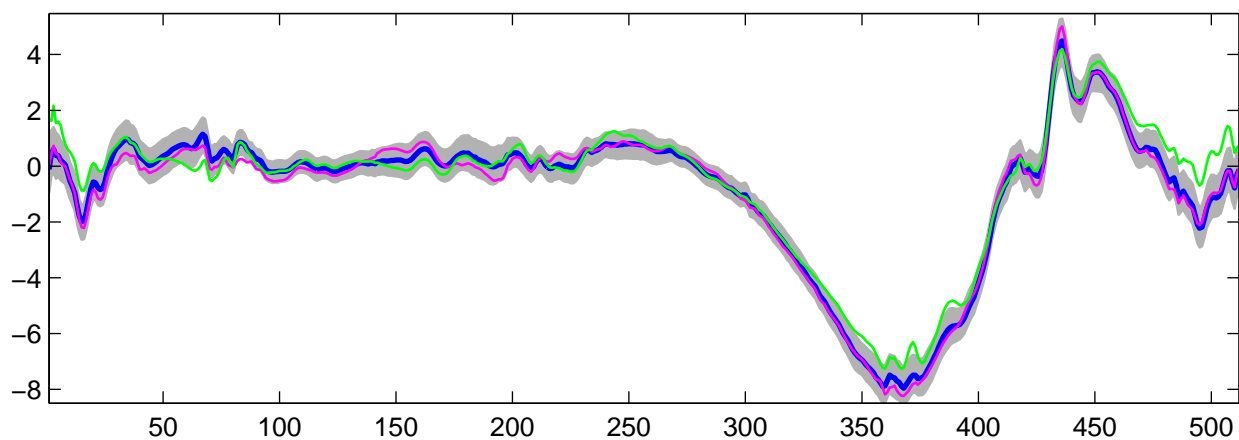
Estimated U_{28}(t) using R-WFMM: t_2 data, run 4
