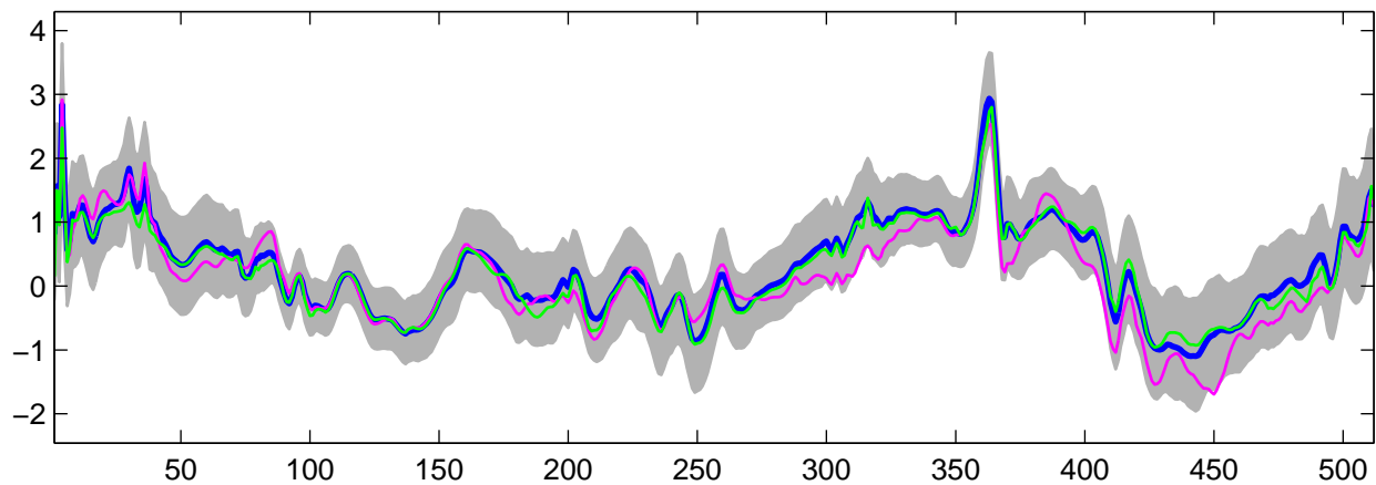
Estimated U_{28}(t) using G-WFMM: t_3 data, run 4
