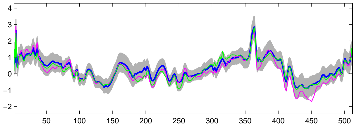
Estimated U_{28}(t) using R-WFMM: t_3 data, run 4
