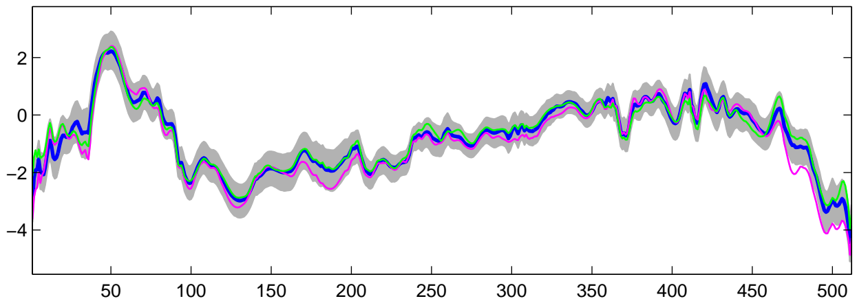
Estimated U_{29}(t) using R-WFMM: DE data, run 4
