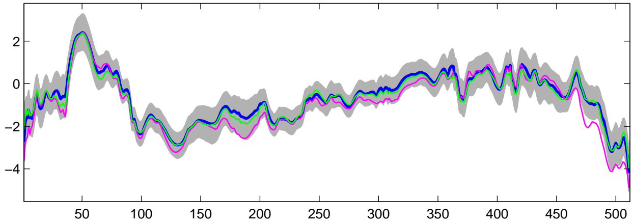
Estimated U_{29}(t) using G-WFMM: DE data, run 4
