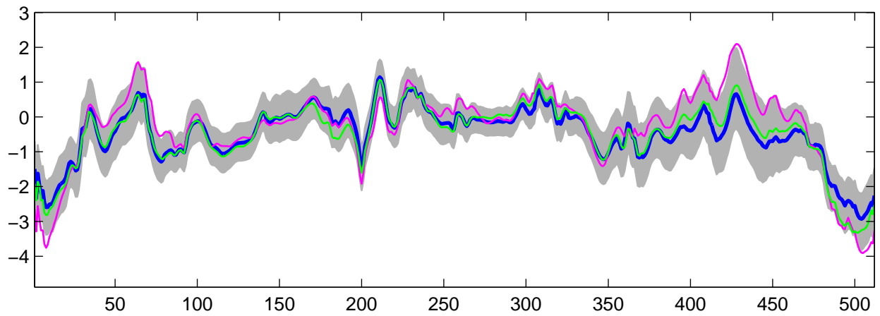
Estimated U_{29}(t) using R-WFMM: Normal data, run 4
