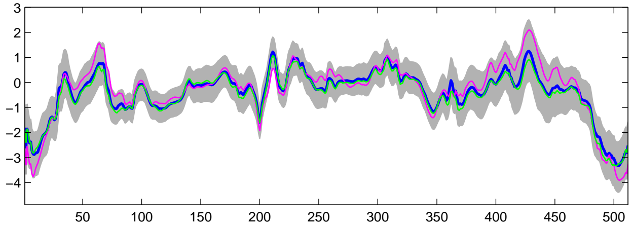
Estimated U_{29}(t) using G-WFMM: Normal data, run 4
