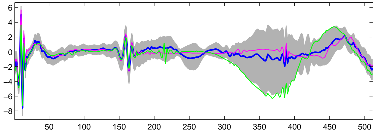
Estimated U_{29}(t) using G-WFMM: t_1 data, run 4
