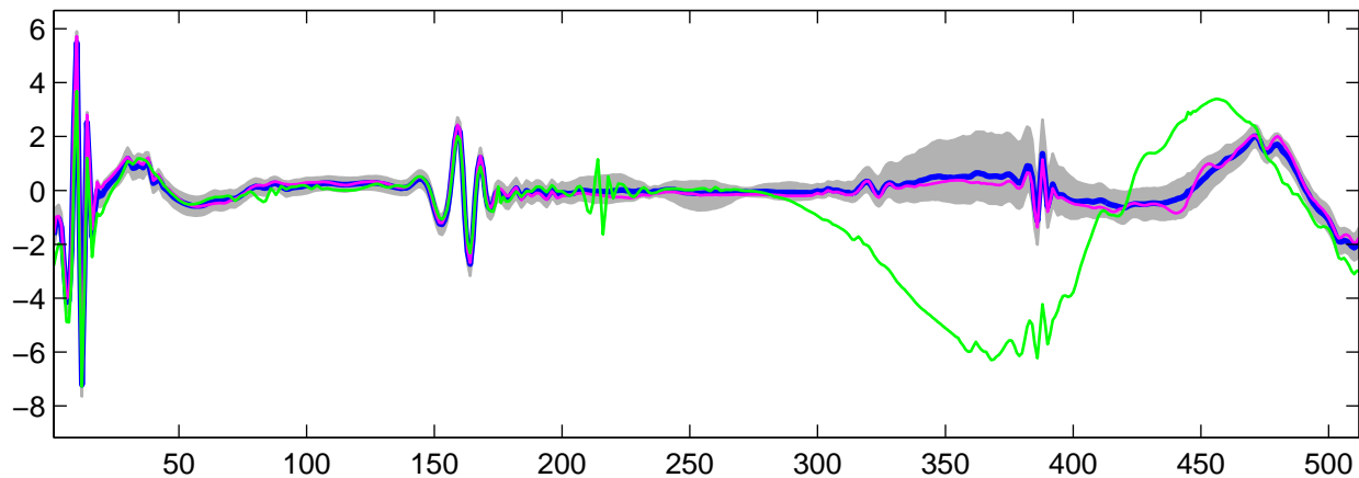
Estimated U_{29}(t) using R-WFMM: t_1 data, run 4
