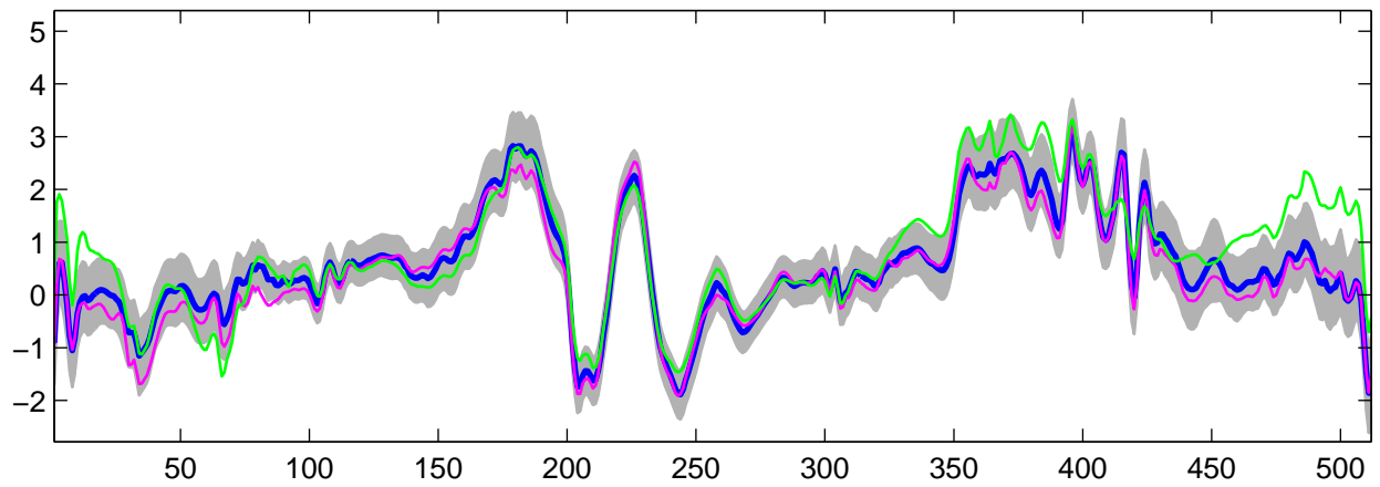
Estimated U_{29}(t) using R-WFMM: t_2 data, run 4
