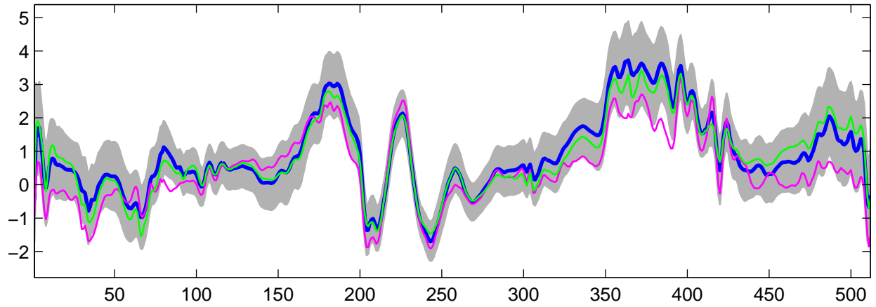
Estimated U_{29}(t) using G-WFMM: t_2 data, run 4
