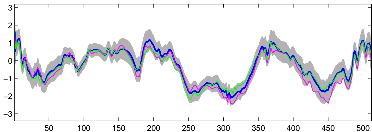
Estimated U_{29}(t) using R-WFMM: t_3 data, run 4
