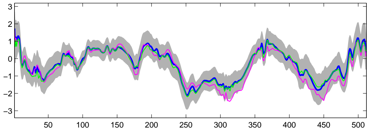
Estimated U_{29}(t) using G-WFMM: t_3 data, run 4
