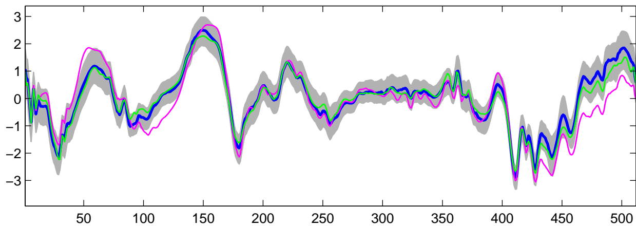
Estimated U_2(t) using R-WFMM: DE data, run 4
