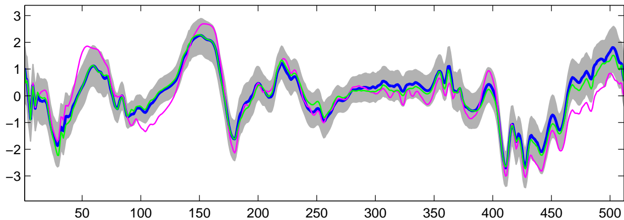
Estimated U_2(t) using G-WFMM: DE data, run 4
