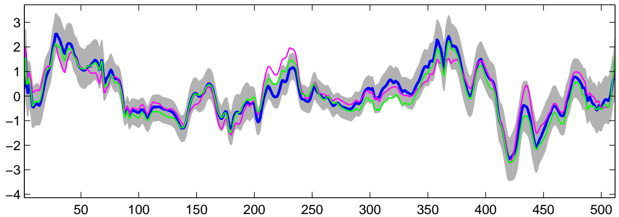
Estimated U_2(t) using R-WFMM: Normal data, run 4
