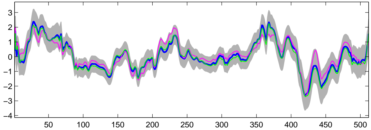
Estimated U_2(t) using G-WFMM: Normal data, run 4
