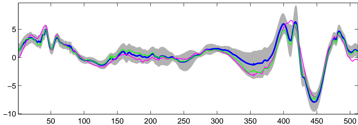
Estimated U_2(t) using G-WFMM: t_1 data, run 4
