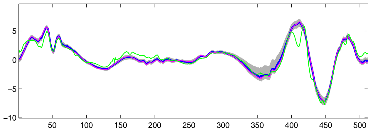
Estimated U_2(t) using R-WFMM: t_1 data, run 4
