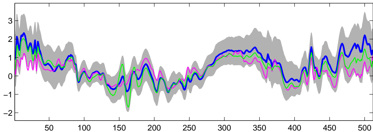
Estimated U_2(t) using G-WFMM: t_2 data, run 4
