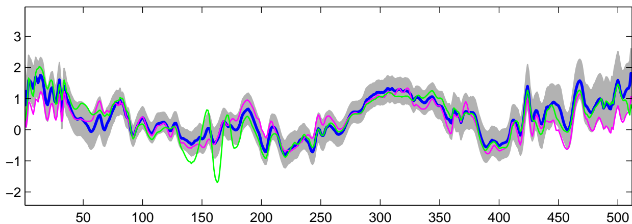
Estimated U_2(t) using R-WFMM: t_2 data, run 4
