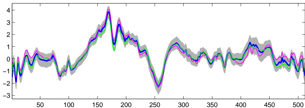
Estimated U_2(t) using R-WFMM: t_3 data, run 4
