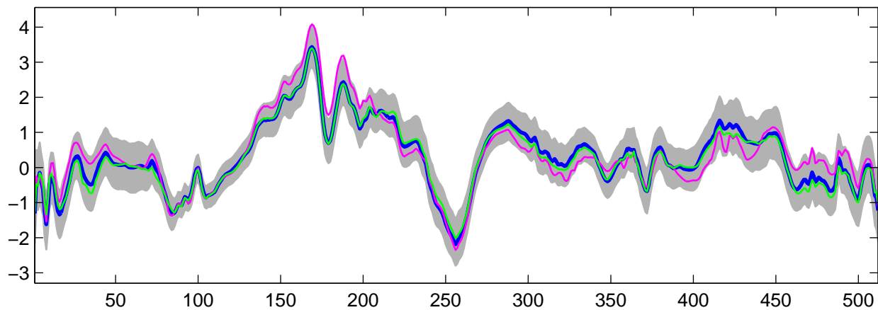
Estimated U_2(t) using G-WFMM: t_3 data, run 4
