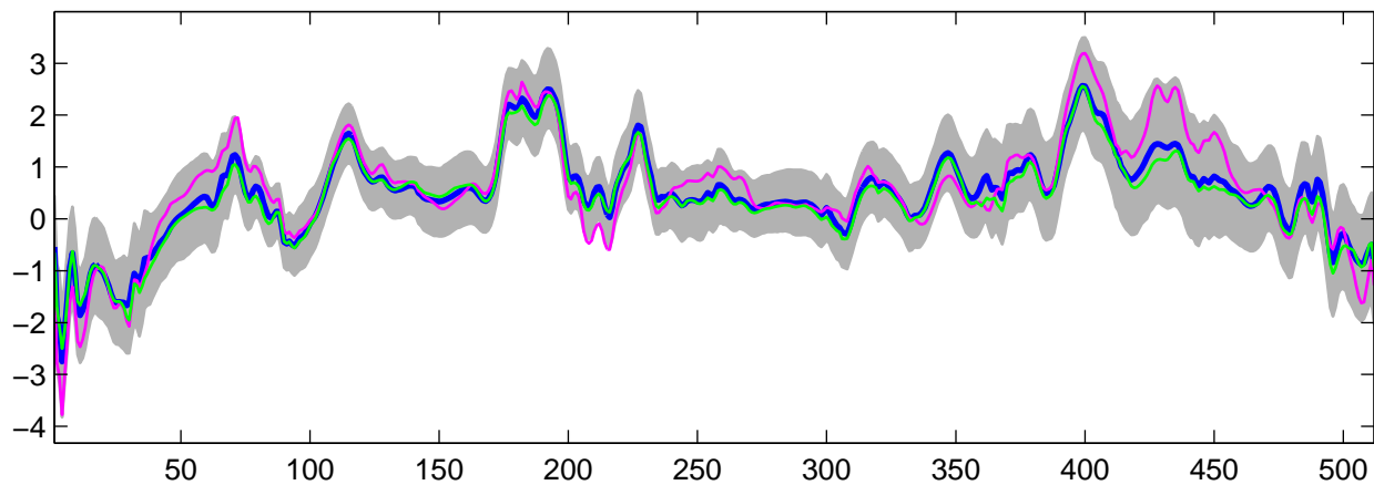
Estimated U_{30}(t) using G-WFMM: Normal data, run 4
