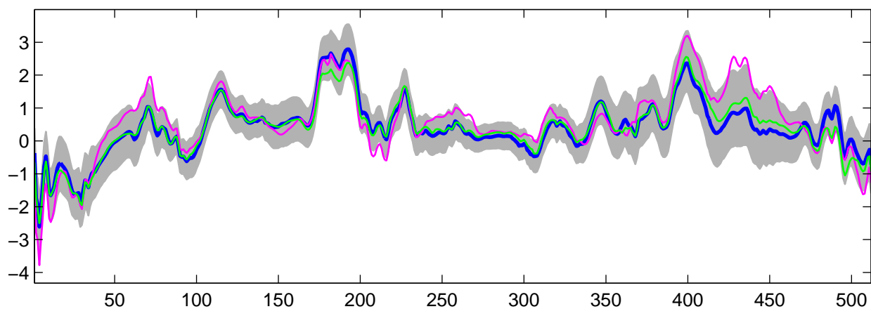
Estimated U_{30}(t) using R-WFMM: Normal data, run 4
