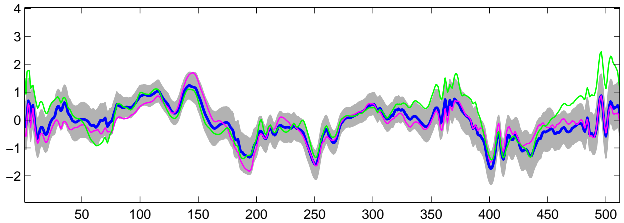
Estimated U_{30}(t) using R-WFMM: t_2 data, run 4
