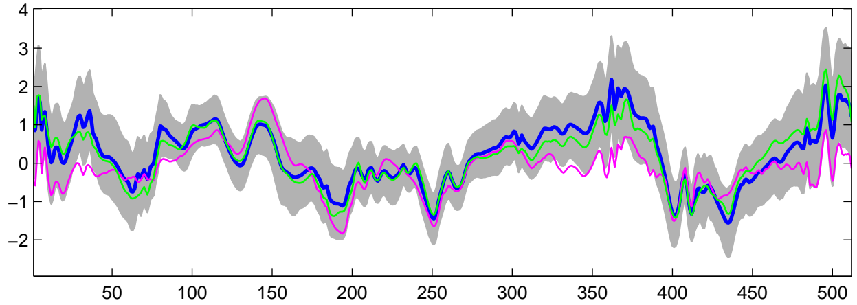
Estimated U_{30}(t) using G-WFMM: t_2 data, run 4
