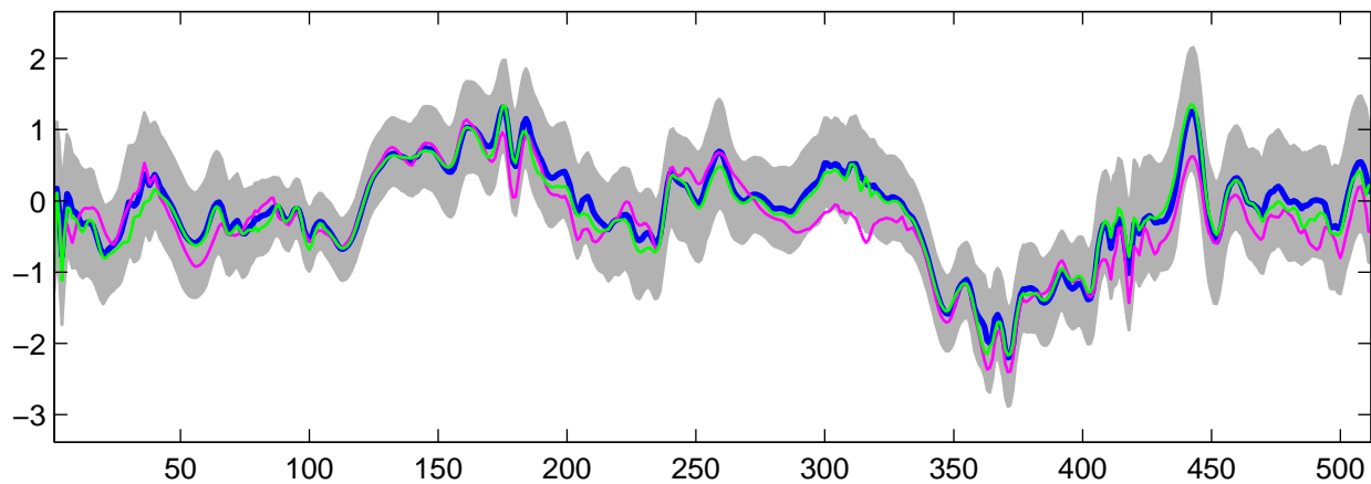
Estimated U_{30}(t) using G-WFMM: t_3 data, run 4
