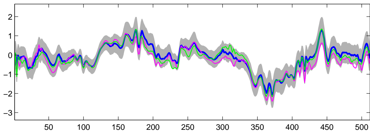
Estimated U_{30}(t) using R-WFMM: t_3 data, run 4
