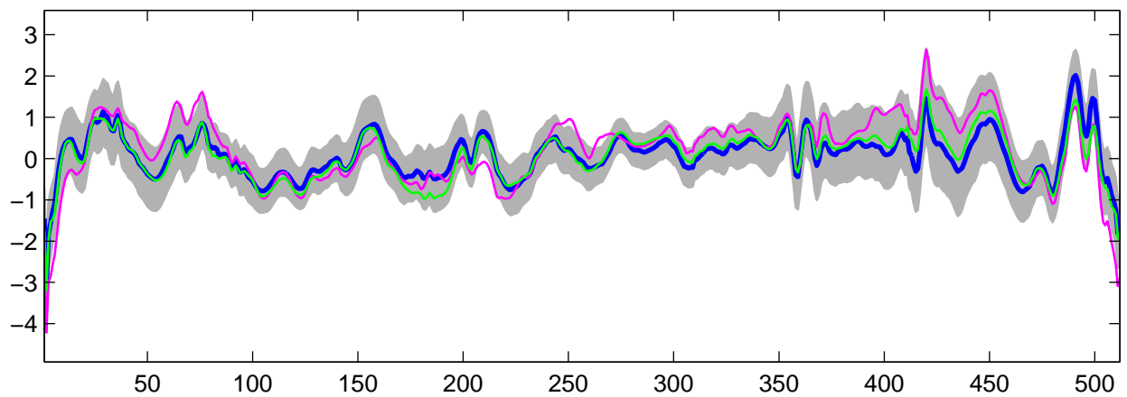
Estimated U_{31}(t) using R-WFMM: Normal data, run 4
