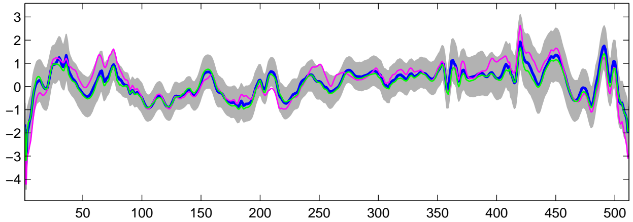
Estimated U_{31}(t) using G-WFMM: Normal data, run 4
