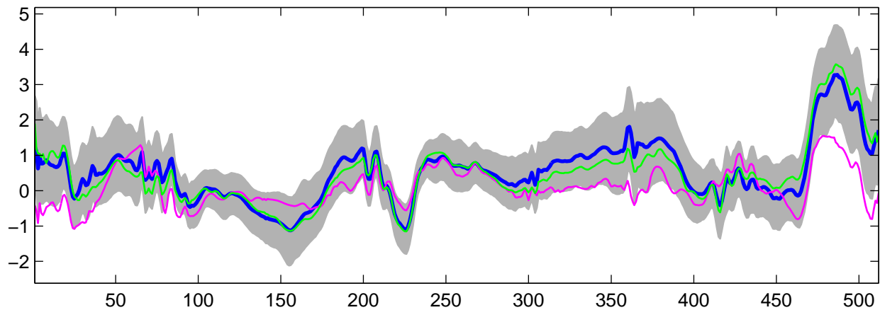
Estimated U_{31}(t) using G-WFMM: t_2 data, run 4
