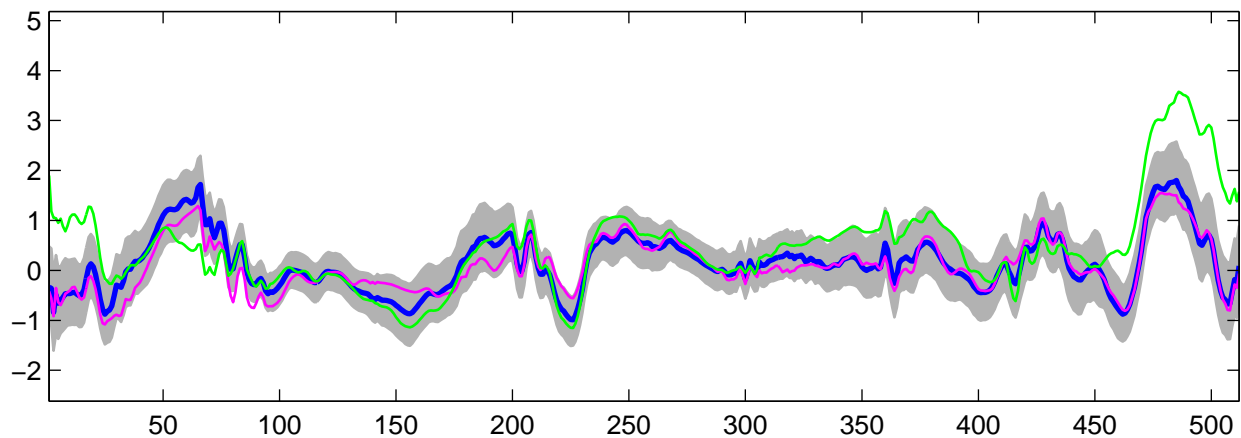
Estimated U_{31}(t) using R-WFMM: t_2 data, run 4
