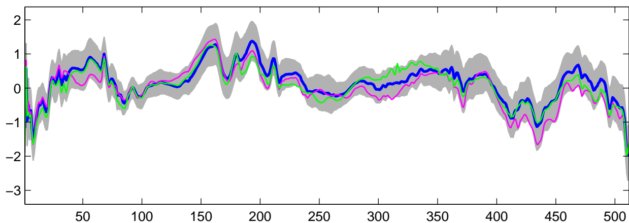
Estimated U_{31}(t) using R-WFMM: t_3 data, run 4
