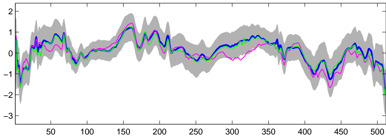
Estimated U_{31}(t) using G-WFMM: t_3 data, run 4
