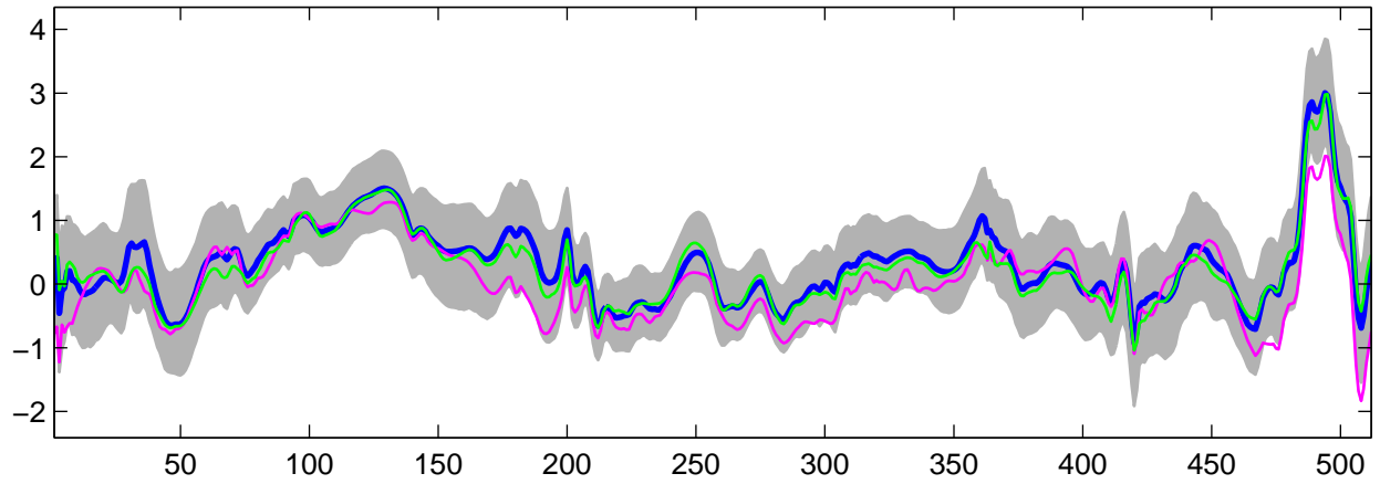
Estimated U_{32}(t) using G-WFMM: DE data, run 4
