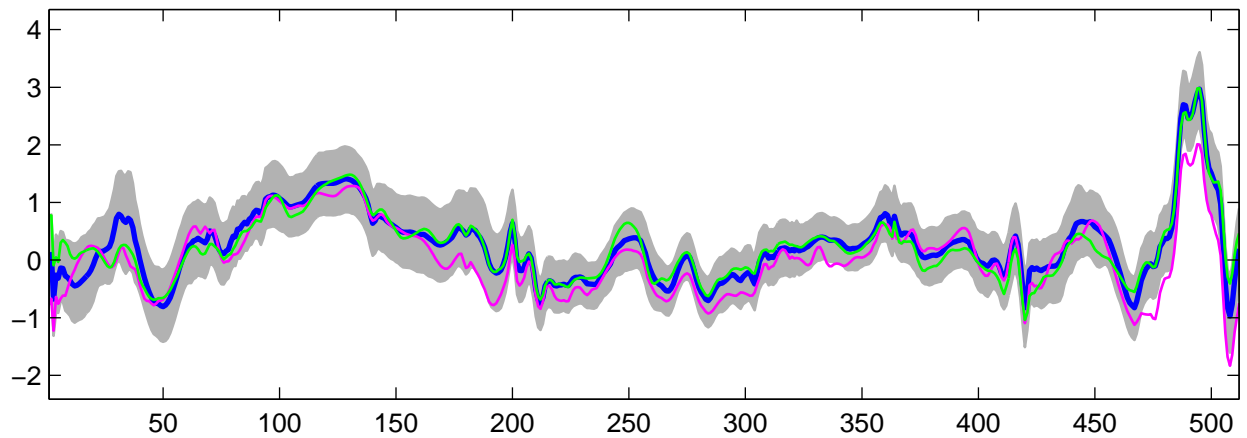
Estimated U_{32}(t) using R-WFMM: DE data, run 4
