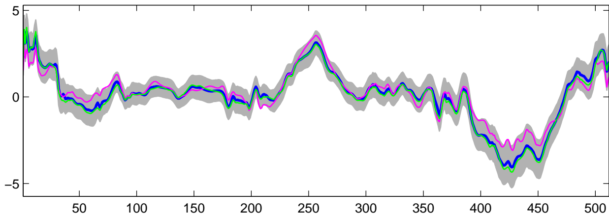
Estimated U_{32}(t) using G-WFMM: Normal data, run 4
