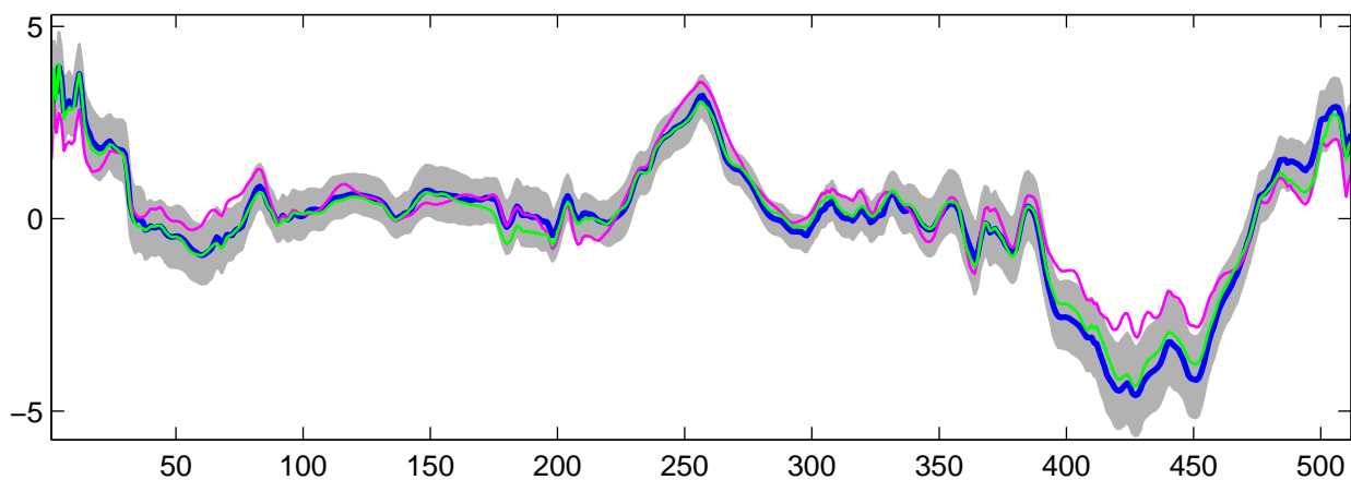
Estimated U_{32}(t) using R-WFMM: Normal data, run 4
