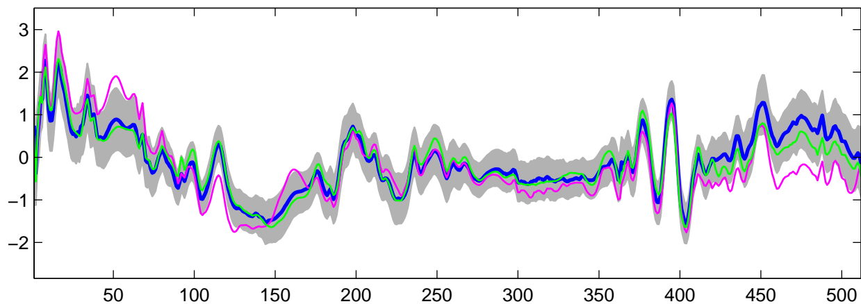
Estimated U_3(t) using R-WFMM: DE data, run 4
