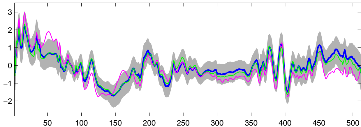
Estimated U_3(t) using G-WFMM: DE data, run 4
