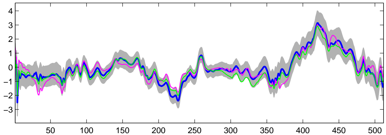
Estimated U_3(t) using R-WFMM: Normal data, run 4
