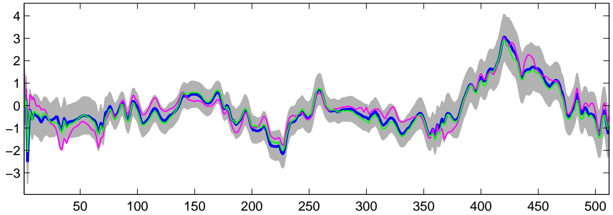
Estimated U_3(t) using G-WFMM: Normal data, run 4
