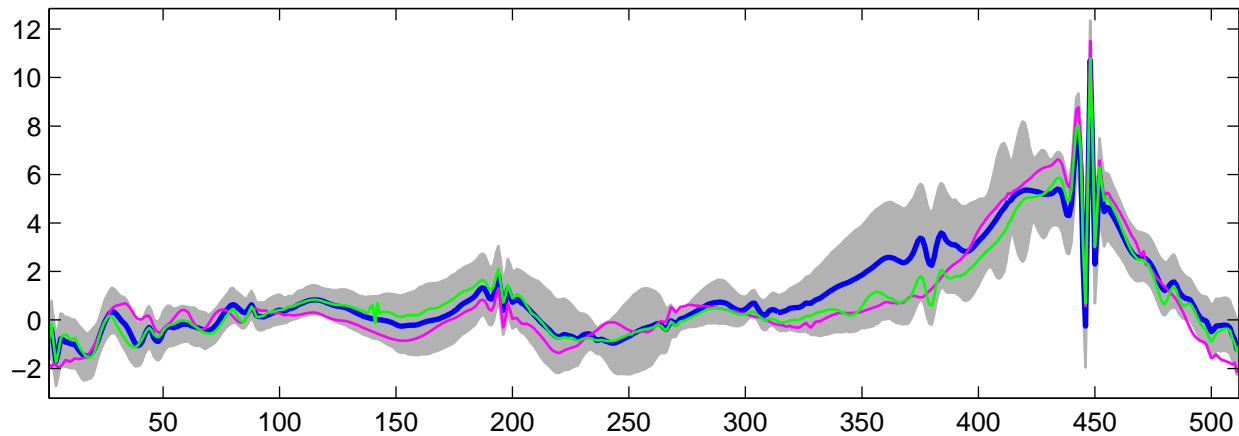
Estimated U_3(t) using G-WFMM: t_1 data, run 4
