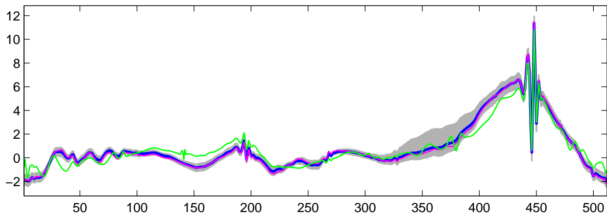
Estimated U_3(t) using R-WFMM: t_1 data, run 4
