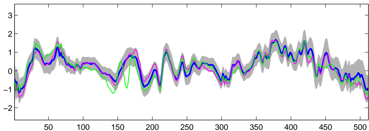
Estimated U_3(t) using R-WFMM: t_2 data, run 4
