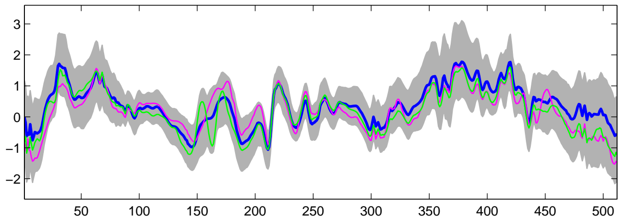
Estimated U_3(t) using G-WFMM: t_2 data, run 4
