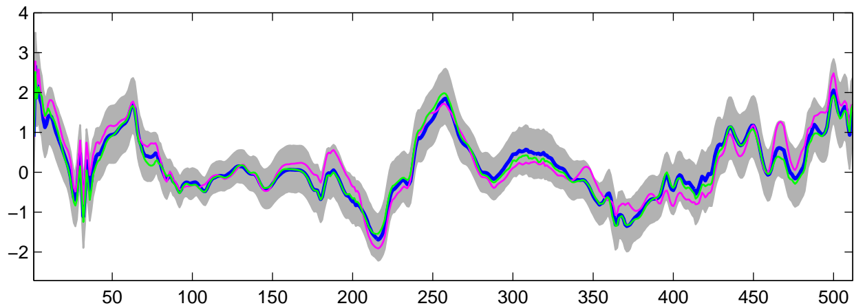
Estimated U_3(t) using G-WFMM: t_3 data, run 4
