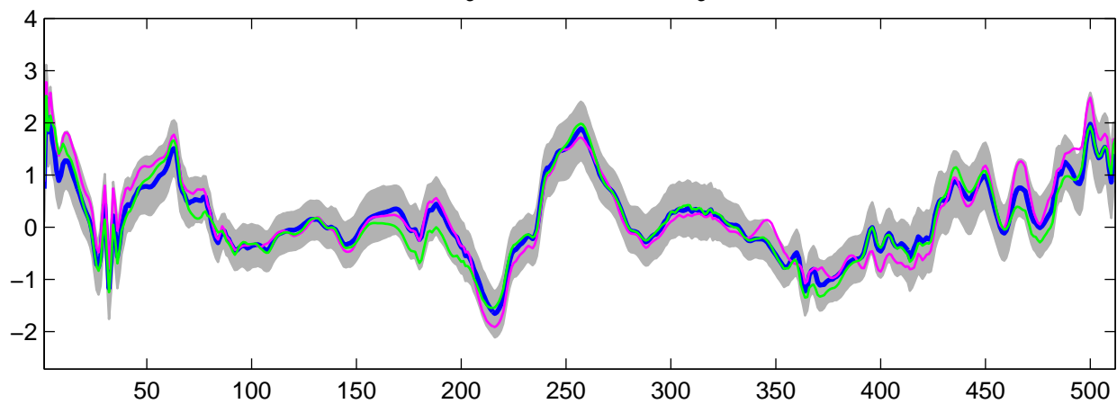
Estimated U_3(t) using R-WFMM: t_3 data, run 4
