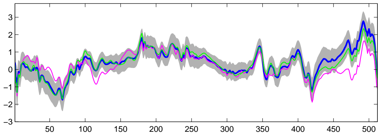
Estimated U_4(t) using R-WFMM: DE data, run 4
