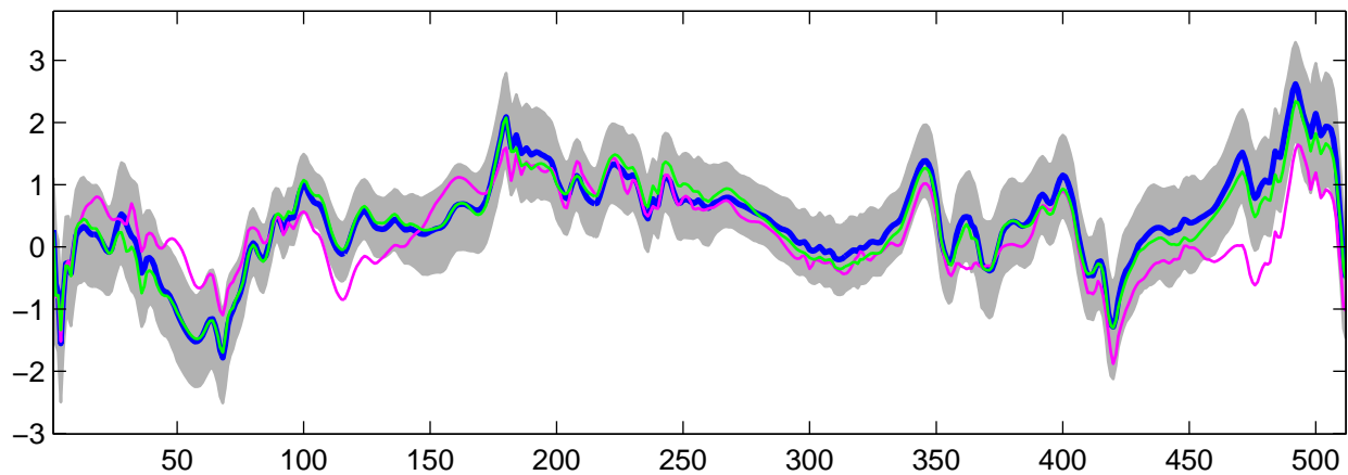
Estimated U_4(t) using G-WFMM: DE data, run 4
