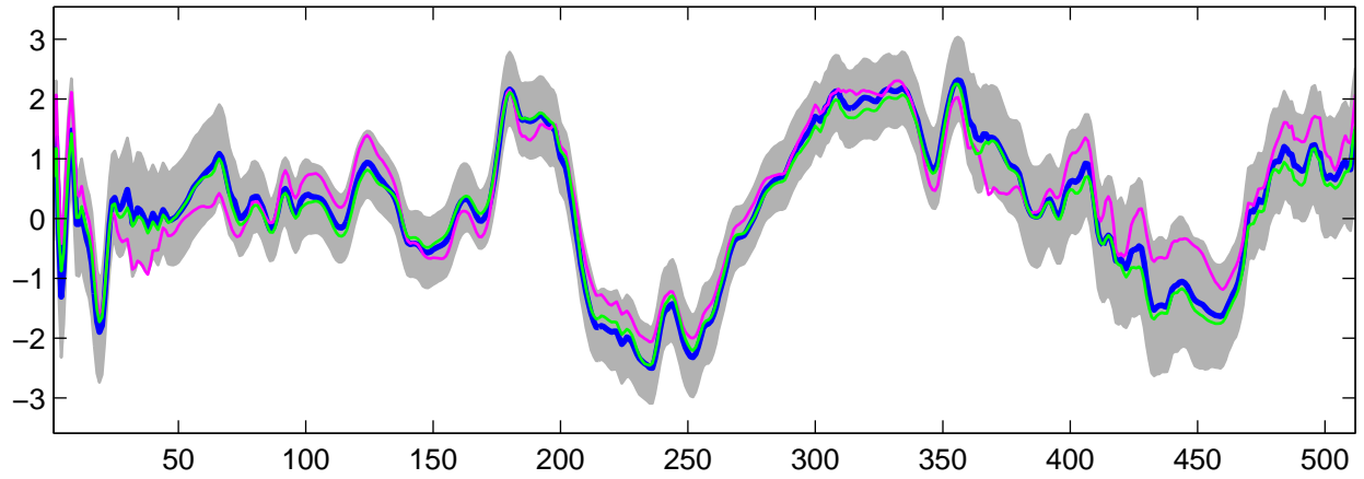
Estimated U_4(t) using G-WFMM: Normal data, run 4
