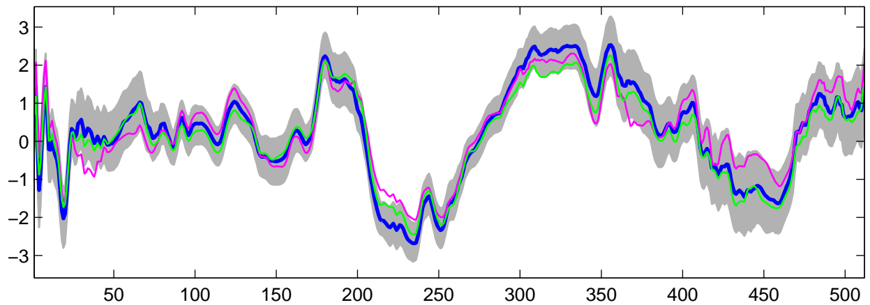
Estimated U_4(t) using R-WFMM: Normal data, run 4
