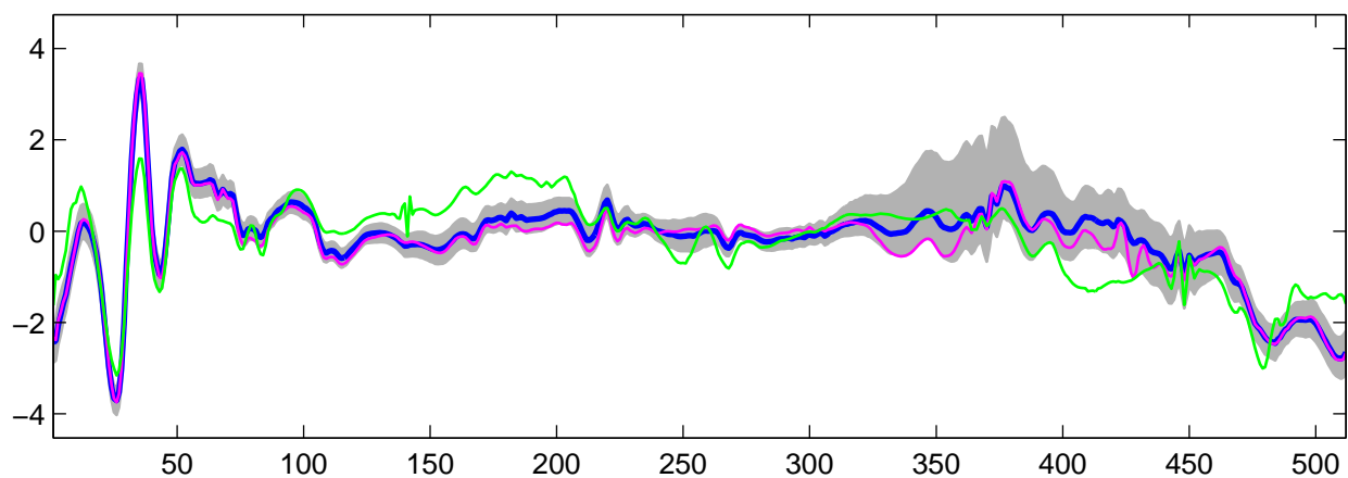
Estimated U_4(t) using R-WFMM: t_1 data, run 4
