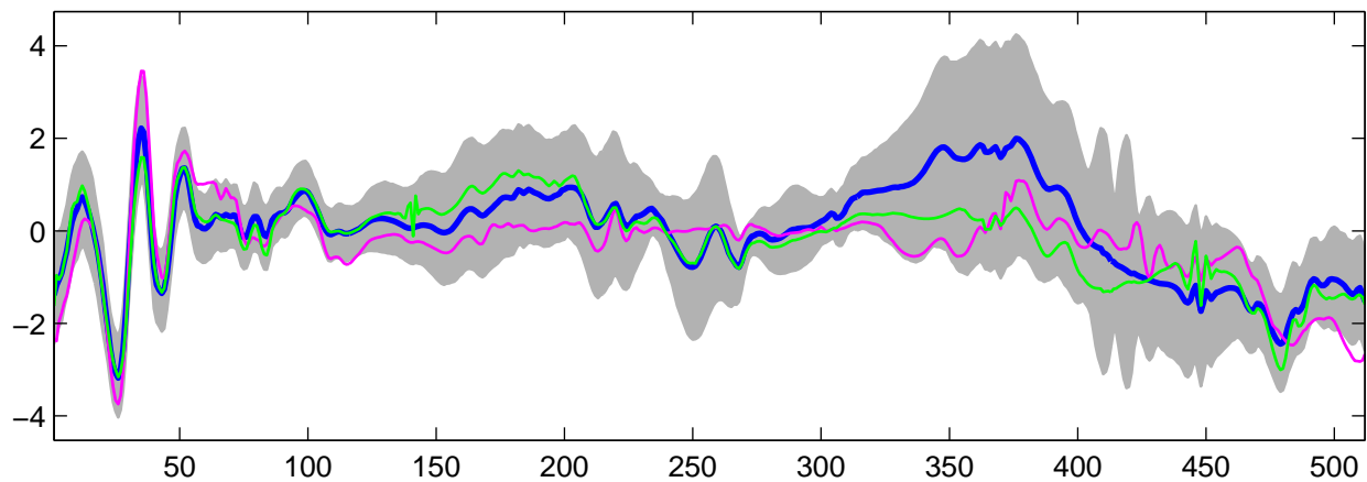
Estimated U_4(t) using G-WFMM: t_1 data, run 4
