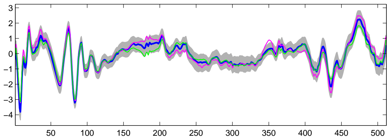
Estimated U_4(t) using R-WFMM: t_3 data, run 4
