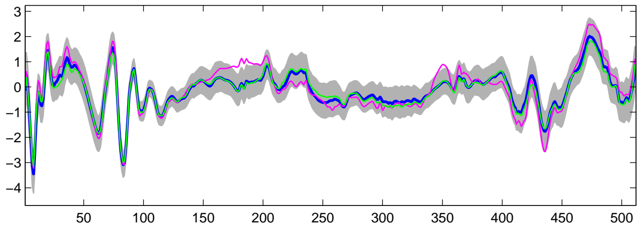
Estimated U_4(t) using G-WFMM: t_3 data, run 4
