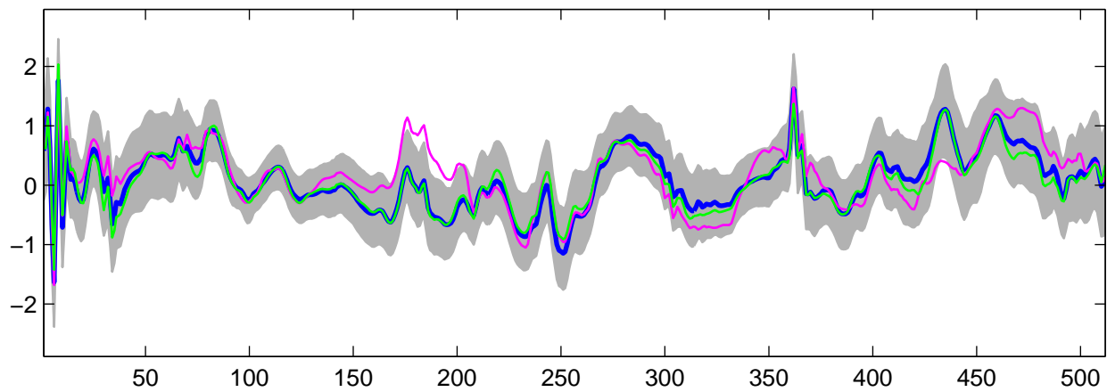
Estimated U_5(t) using G-WFMM: t_3 data, run 4
