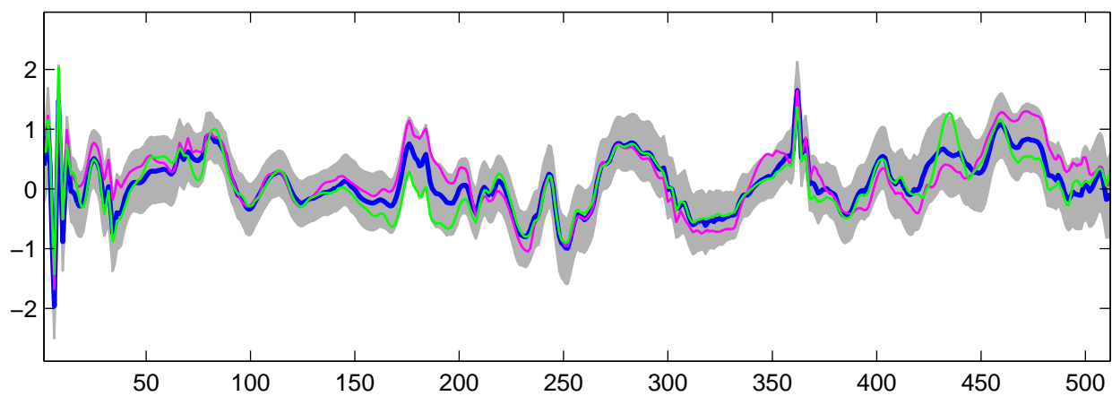
Estimated U_5(t) using R-WFMM: t_3 data, run 4
