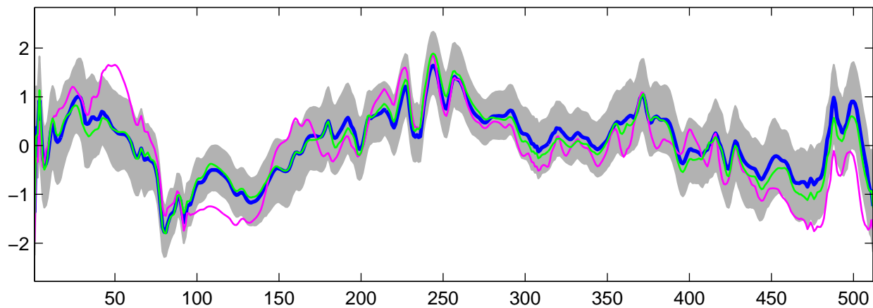
Estimated U_6(t) using G-WFMM: DE data, run 4
