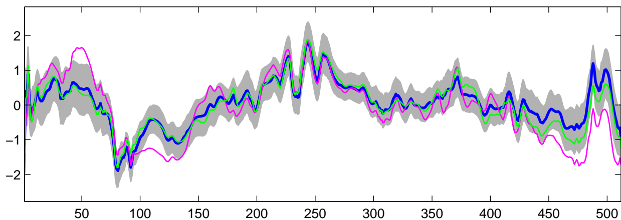
Estimated U_6(t) using R-WFMM: DE data, run 4
