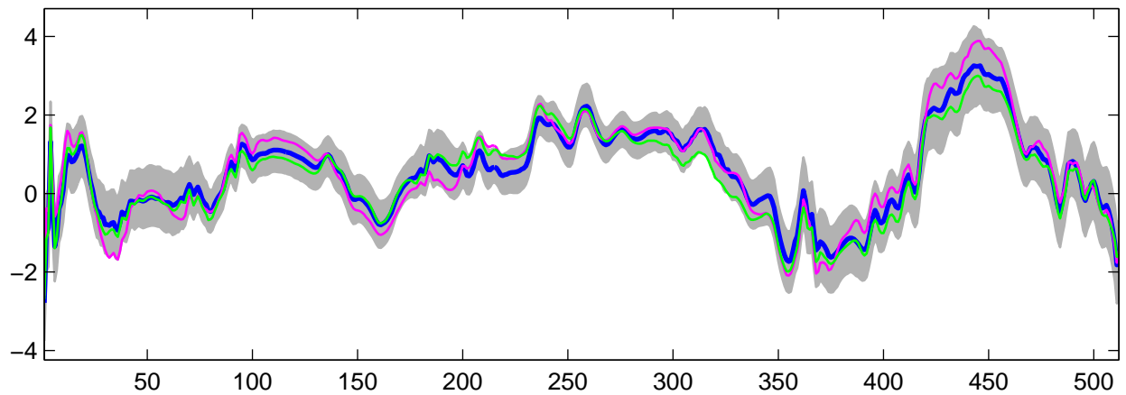
Estimated U_6(t) using R-WFMM: Normal data, run 4
