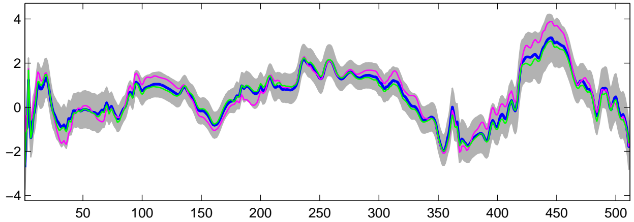
Estimated U_6(t) using G-WFMM: Normal data, run 4
