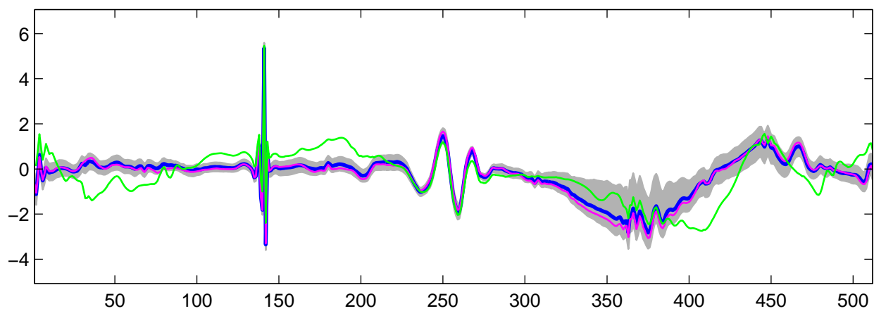
Estimated U_{\hat{\theta}}(t) using R-WFMM: t_1 data, run 4
