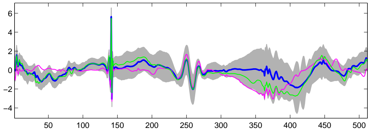
Estimated U_{\hat{\theta}}(t) using G-WFMM: t_1 data, run 4
