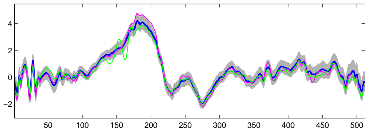
Estimated U_6(t) using R-WFMM: t_2 data, run 4
