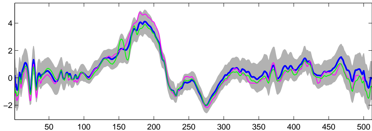
Estimated U_6(t) using G-WFMM: t_2 data, run 4
