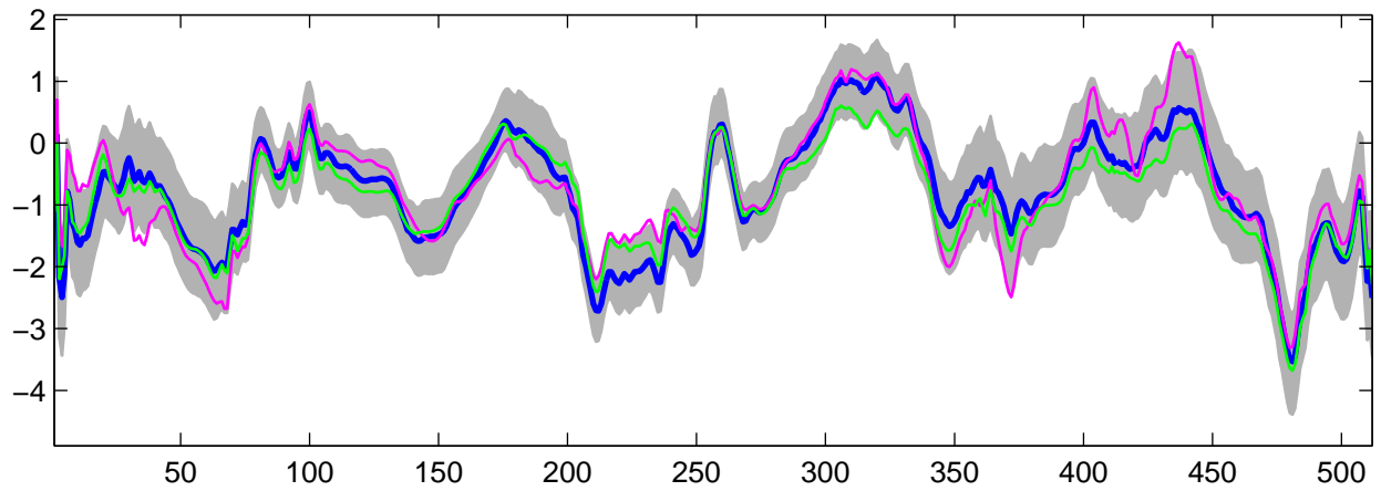
Estimated U_7(t) using R-WFMM: Normal data, run 4
