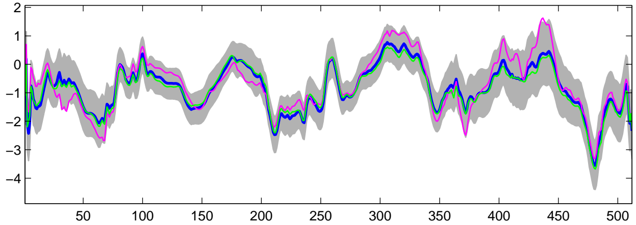
Estimated U_7(t) using G-WFMM: Normal data, run 4
