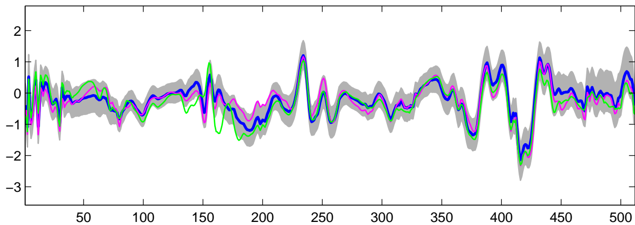
Estimated U_7(t) using R-WFMM: t_2 data, run 4
