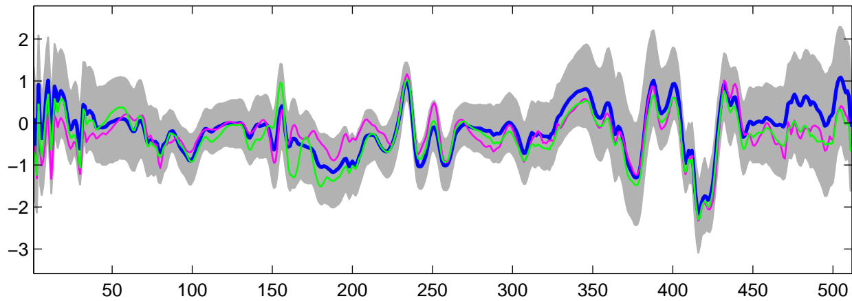
Estimated U_7(t) using G-WFMM: t_2 data, run 4
