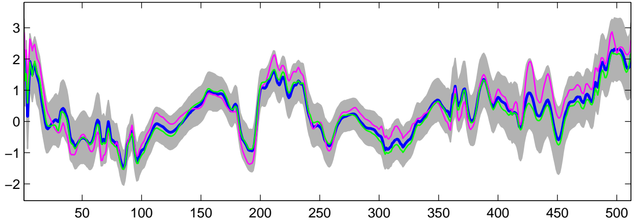
Estimated U_g(t) using G-WFMM: Normal data, run 4
