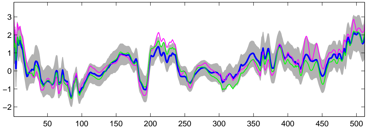
Estimated U_g(t) using R-WFMM: Normal data, run 4
