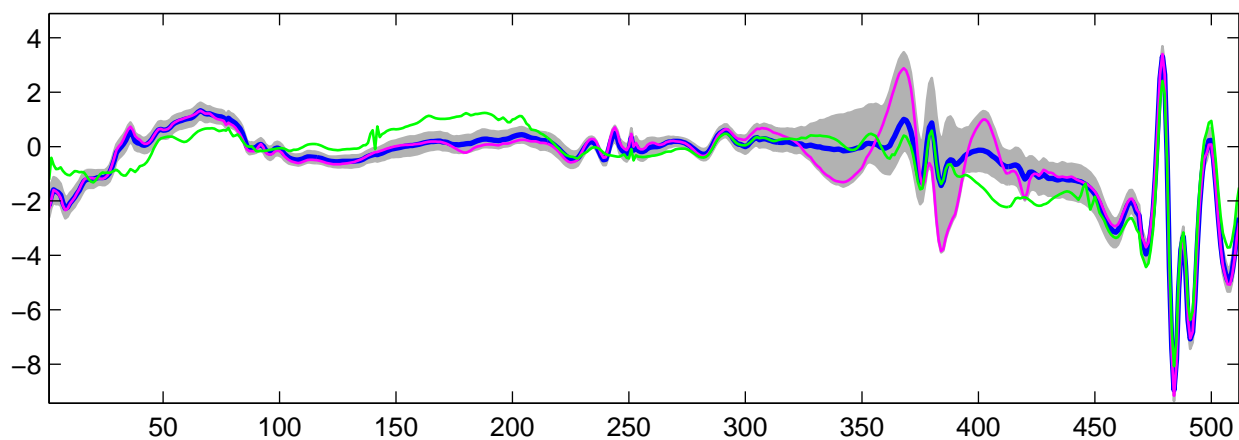
Estimated U_8(t) using R-WFMM: t_1 data, run 4
