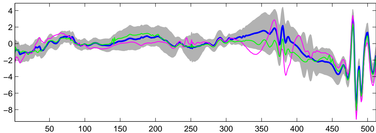
Estimated U_8(t) using G-WFMM: t_1 data, run 4
