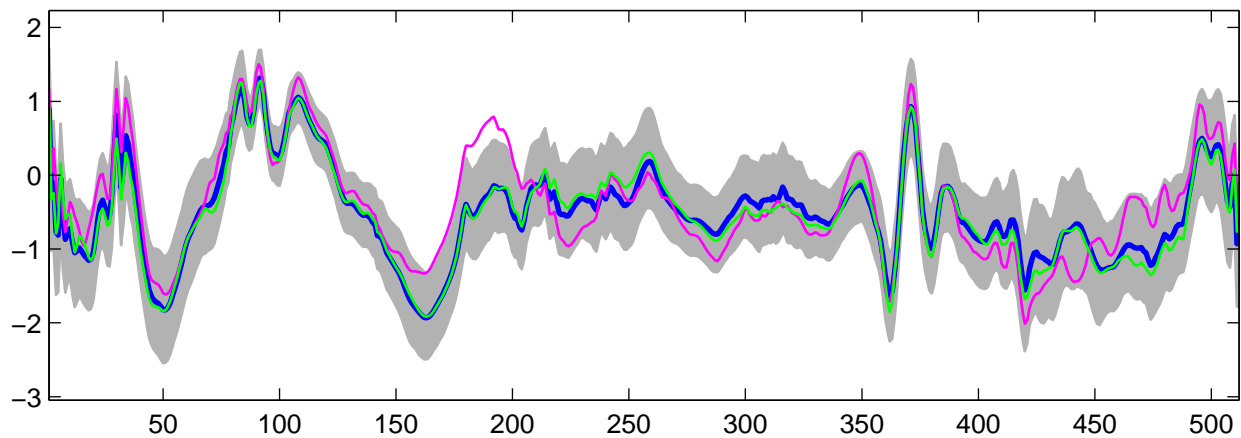
Estimated U_8(t) using G-WFMM: t_3 data, run 4
