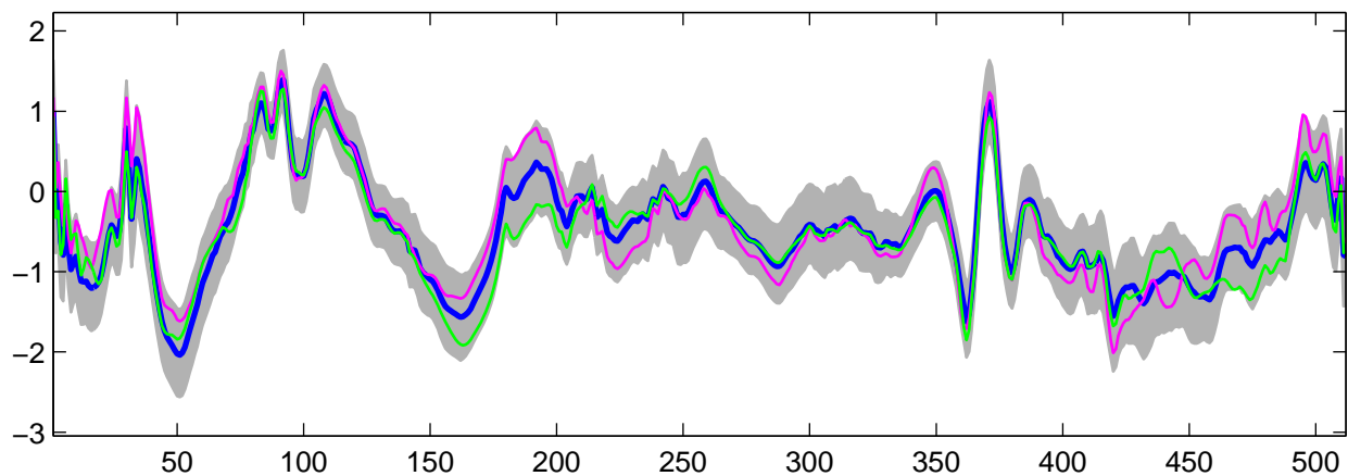
Estimated U_8(t) using R-WFMM: t_3 data, run 4
