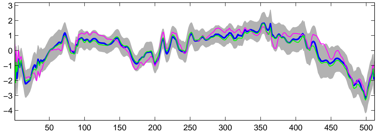
Estimated U_{\theta}(t) using G-WFMM: Normal data, run 4
