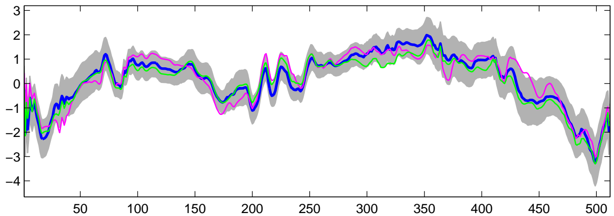
Estimated U_{\theta}(t) using R-WFMM: Normal data, run 4
