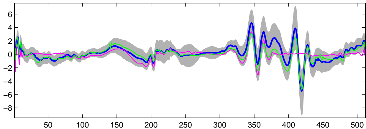
Estimated U_{\theta}(t) using G-WFMM: t_1 data, run 4
