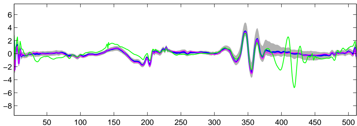
Estimated U_{\theta}(t) using R-WFMM: t_1 data, run 4
