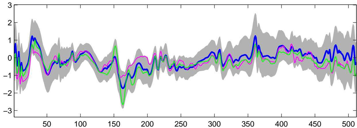
Estimated U_\theta(t) using G-WFMM: t_2 data, run 4
