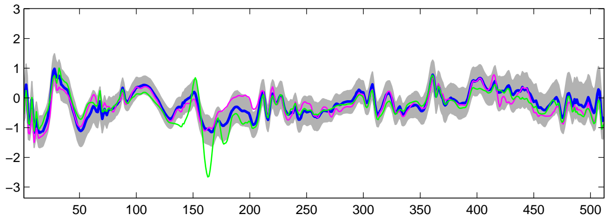
Estimated U_\theta(t) using R-WFMM: t_2 data, run 4
