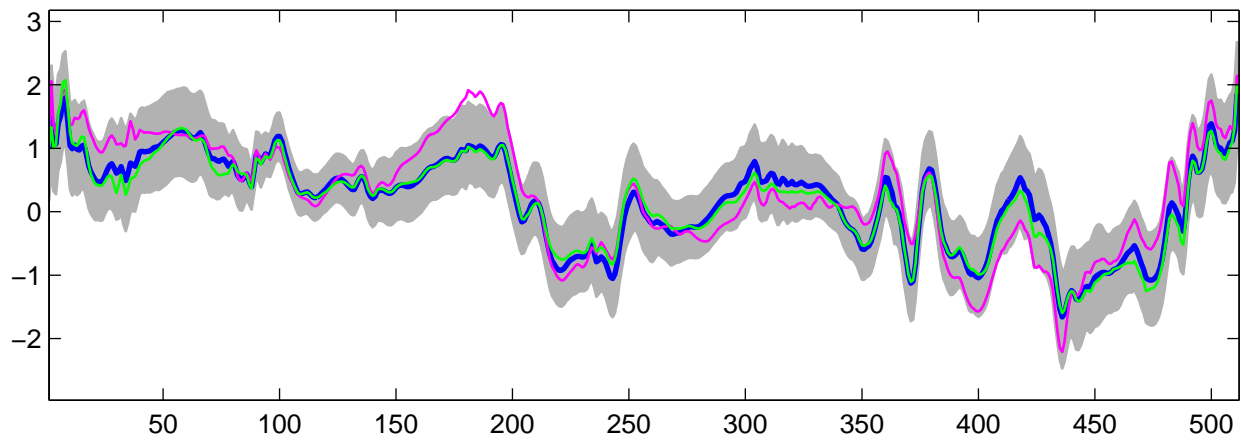
Estimated U_9(t) using G-WFMM: t_3 data, run 4
