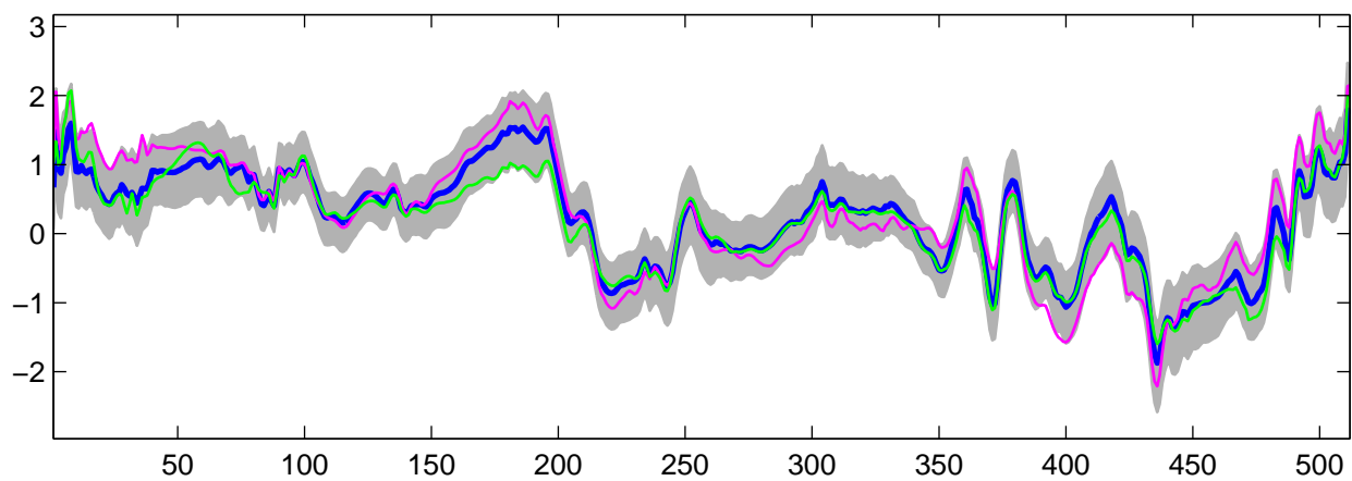
Estimated U_9(t) using R-WFMM: t_3 data, run 4
