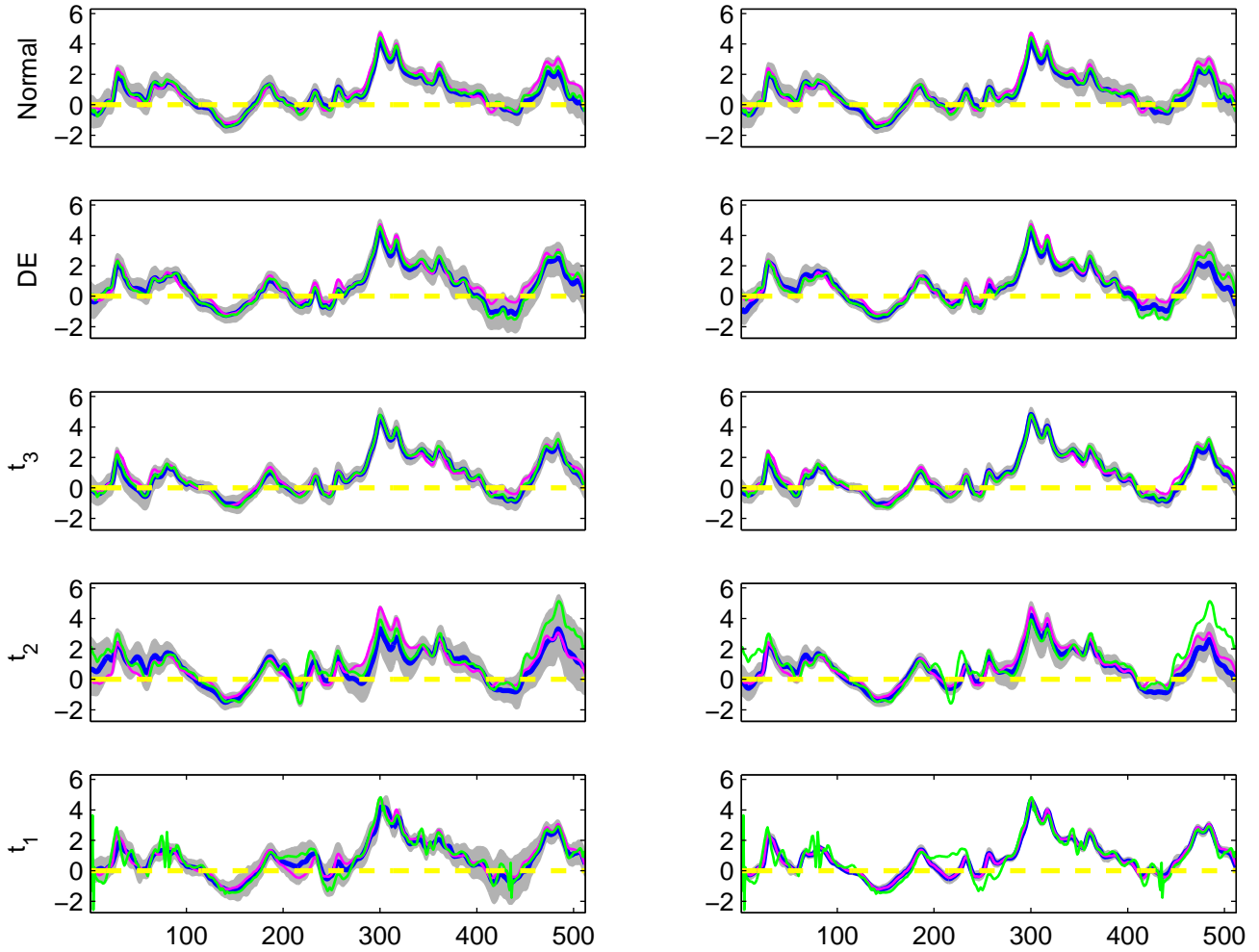
The estimated B_1(t) for 5 simulated datasets, simulation run 5 G-WFMM R-WFMM
