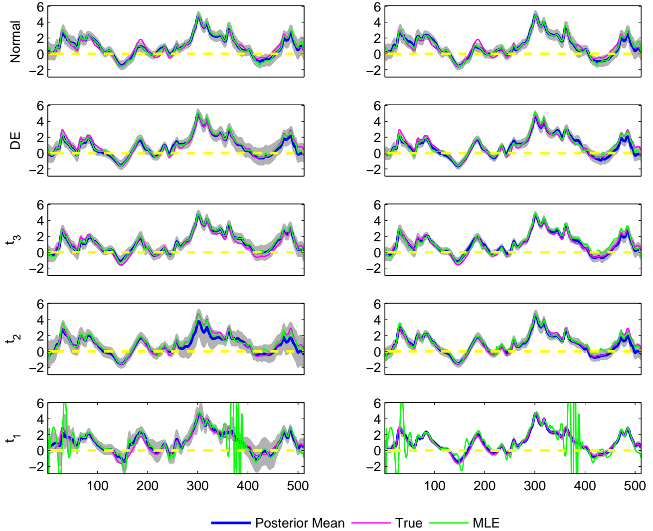
The estimated B_2(t) for 5 simulated datasets, simulation run 5
