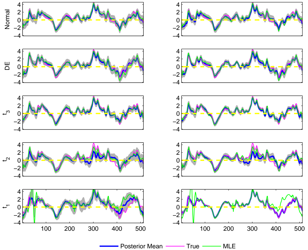
The estimated B_3(t) for 5 simulated datasets, simulation run 5
