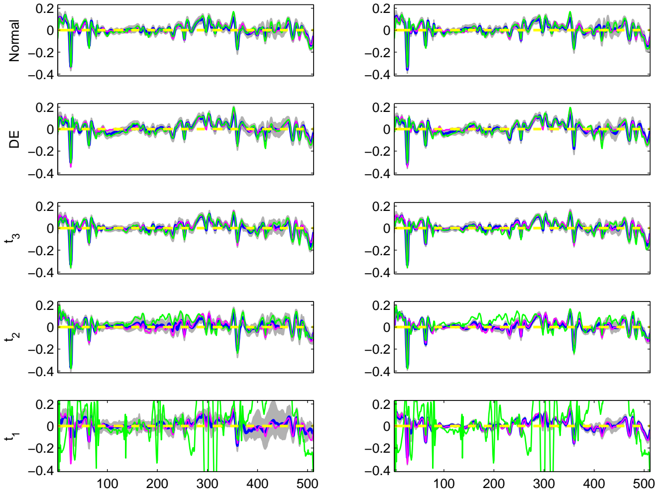
The estimated B_5(t) for 5 simulated datasets, simulation run 5 G-WFMM R-WFMM
